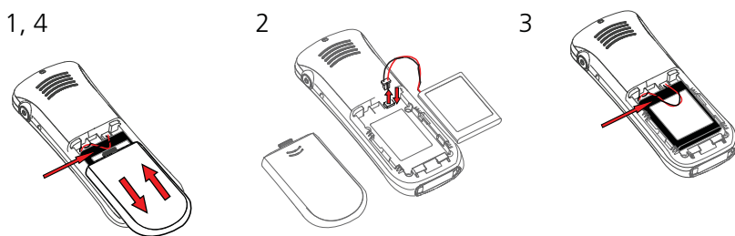
Figure 6: Battery replacement
